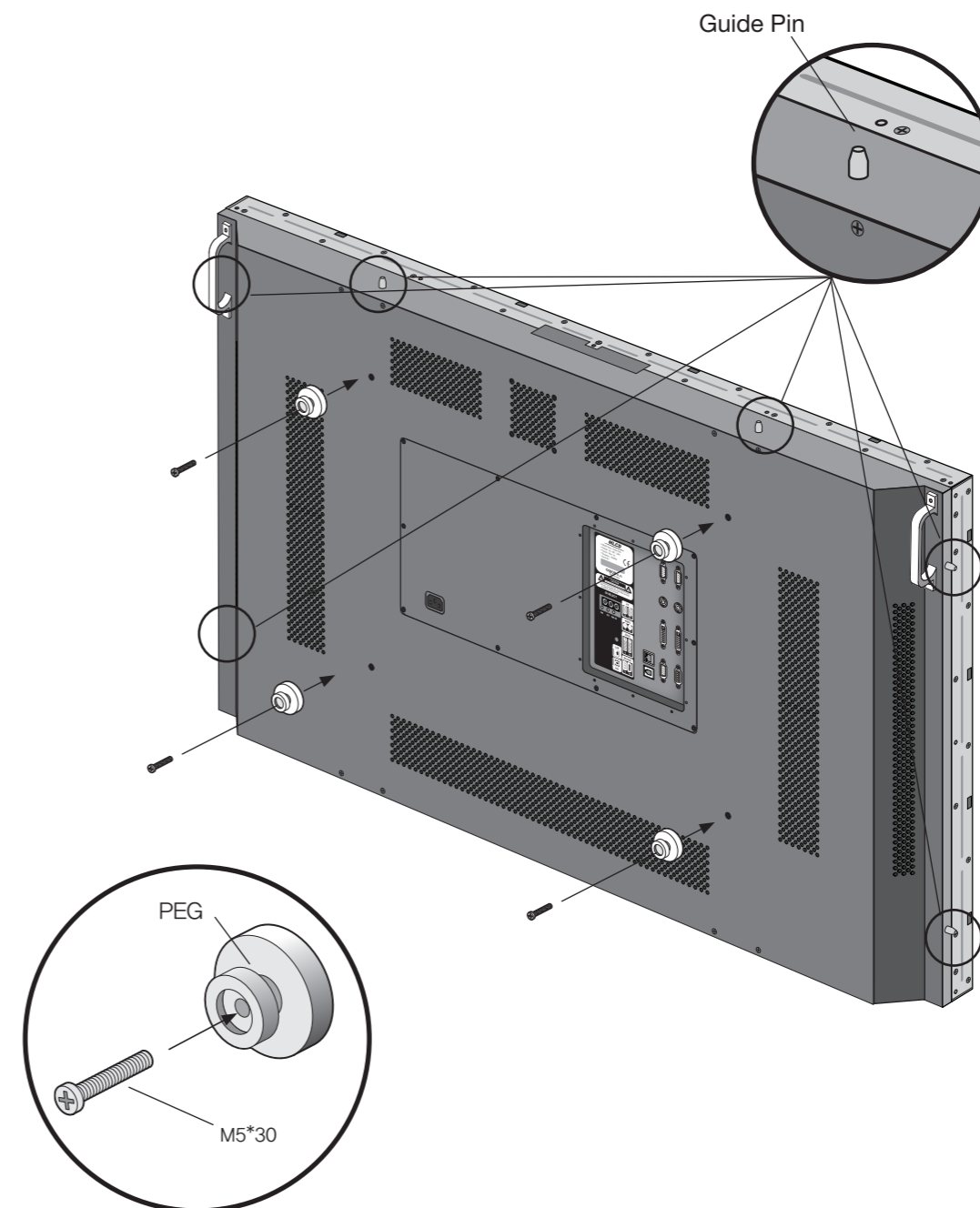
Fasten 4 PEGs in the back of MLCD with M5*30 bolts.
