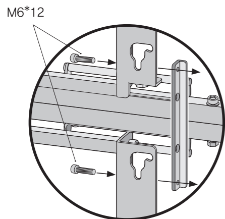
Connect the Main Frame and "Y-Axis Link" with M6*12 bolts using a 5mm allen wrench.
