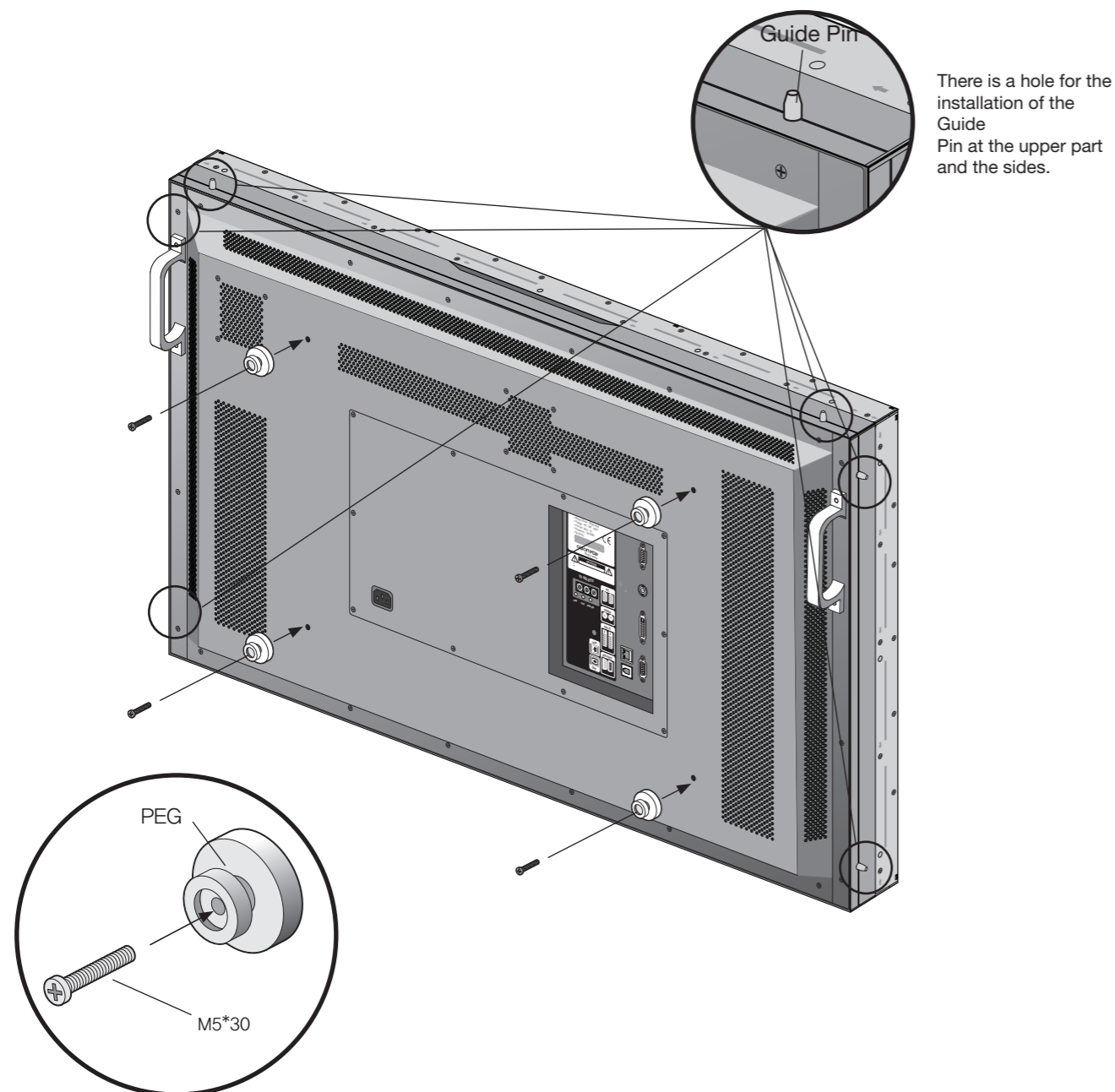
Fasten 4 PEGs in the back of MLCD with M5*30 bolts.
