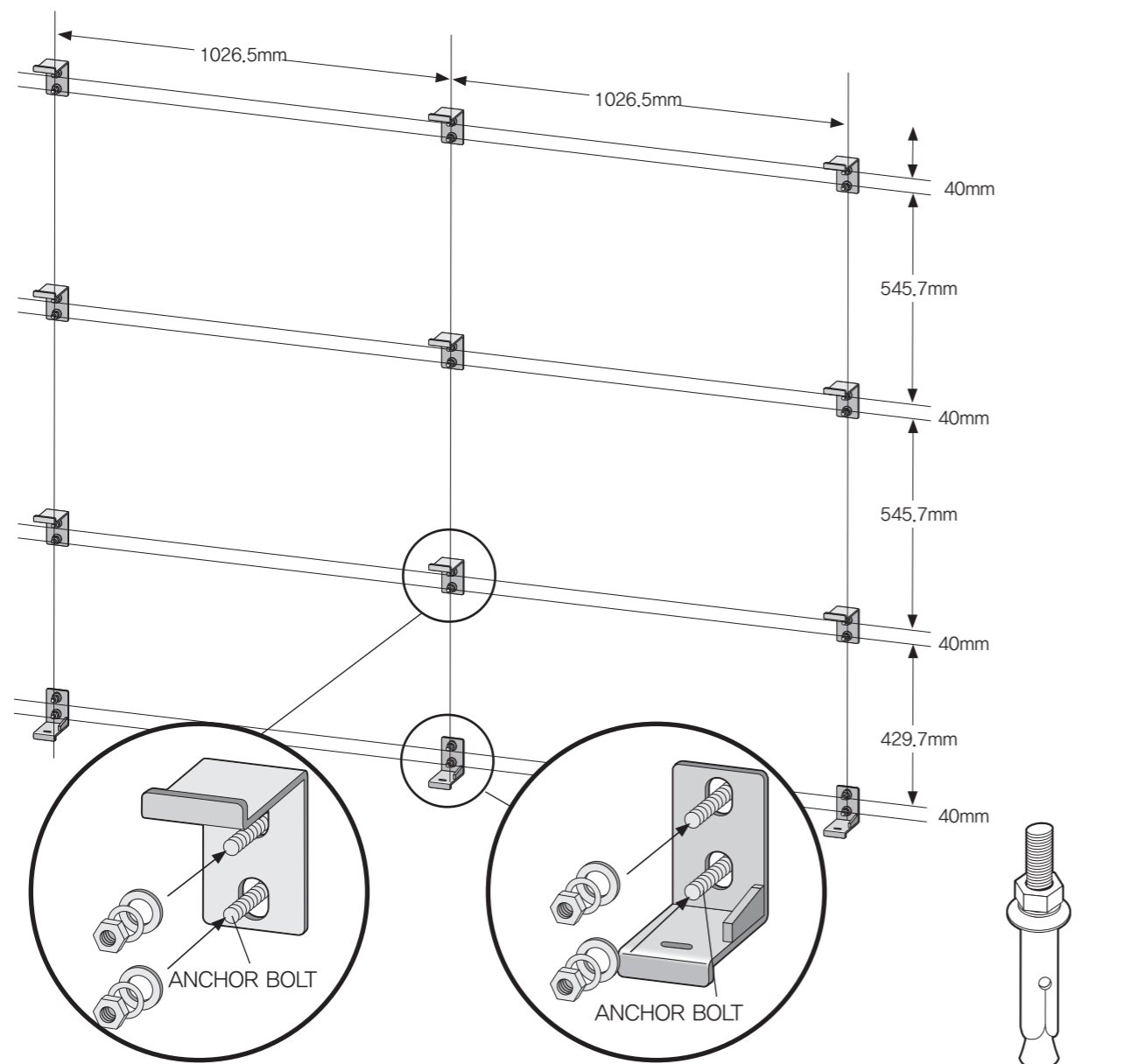
Attach the anchor bolts (3/8") and Wall Brackets into the wall.
