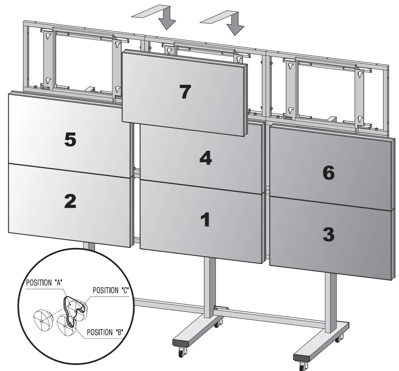
If you need to detach a MLCD set in the lower line, move the set in the upper line to position "C". Remove guide pins from the set in the lower line, move it to position "A" and detach from the main frame.
