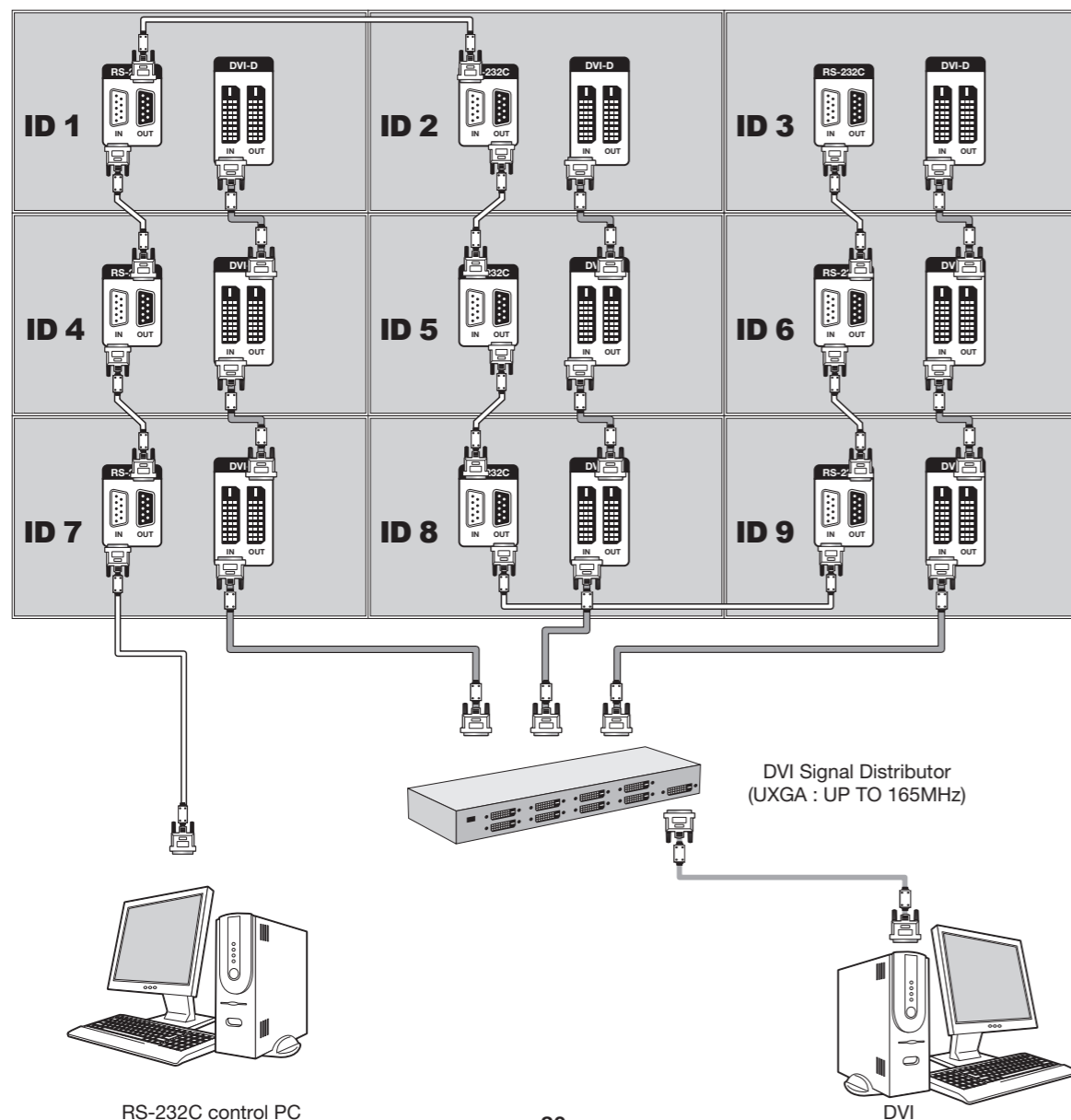
RS-232C control PC
