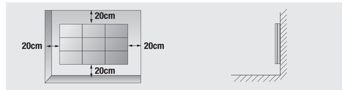
Mount on the MAIN FRAME wall Please secure minimum clearance as shown in the picture for adequate ventilation and technical service.
