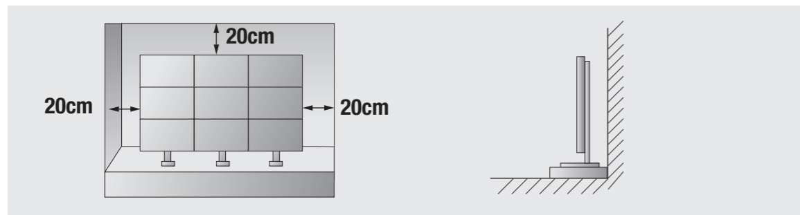
Install on a MAIN FRAME Stand Please secure minimum clearance as shown in the picture for adequate ventilation and technical service.
